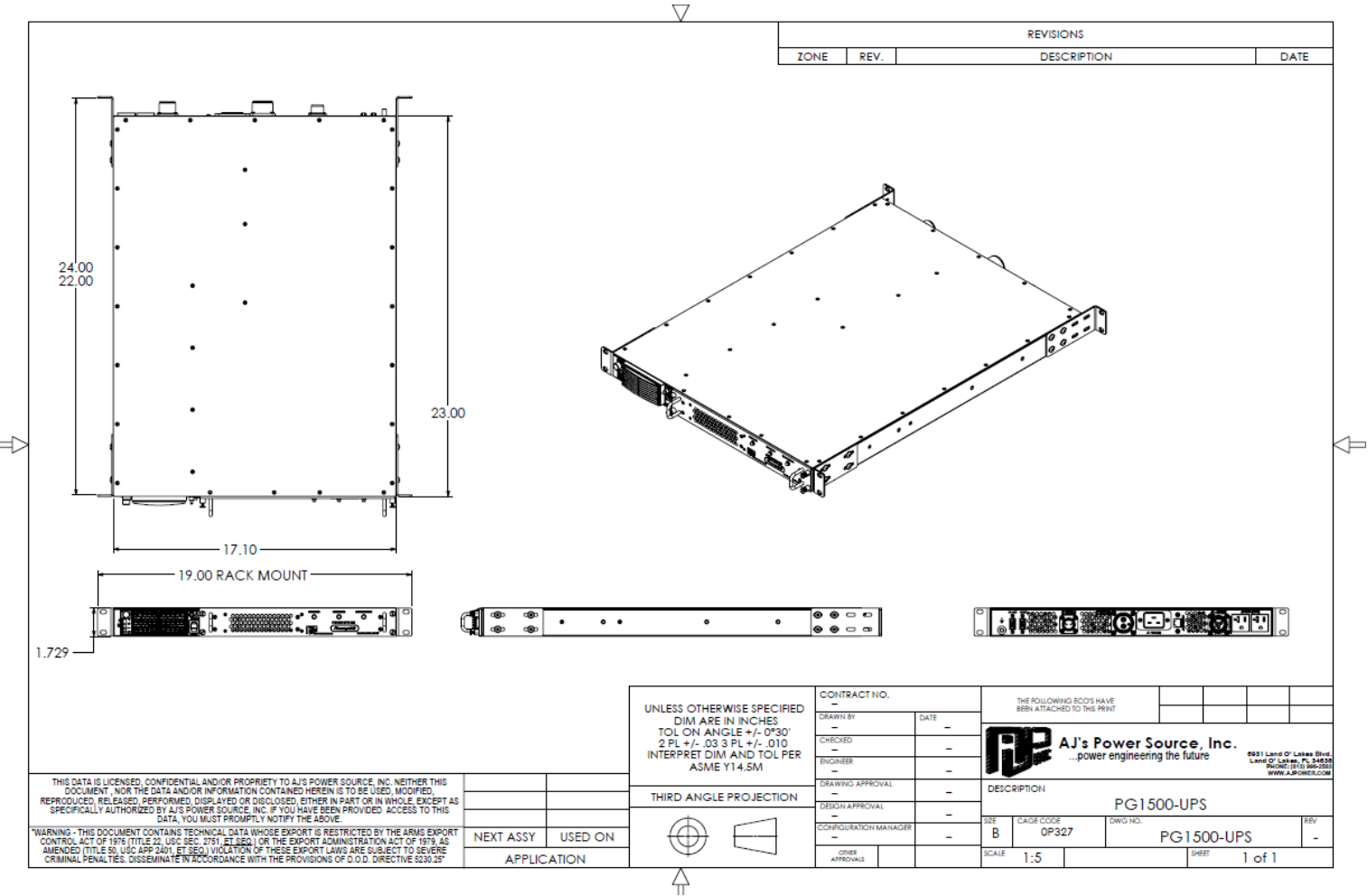
Mechanical Drawing (PG1500-UPS shown, PG1500-UPS-230-NG similar)
