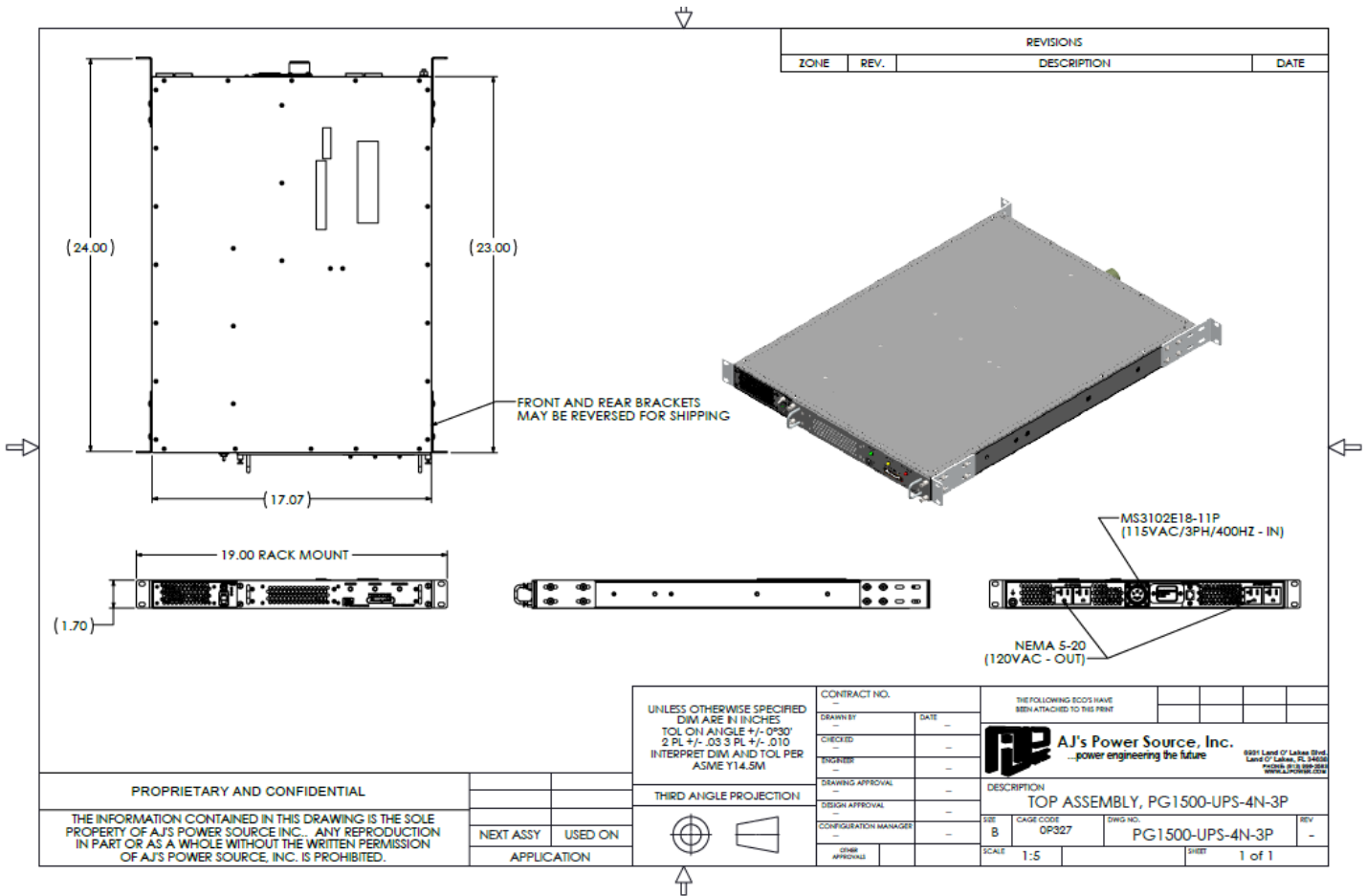
PG1500-UPS-4N-3P Mechanical Drawing
