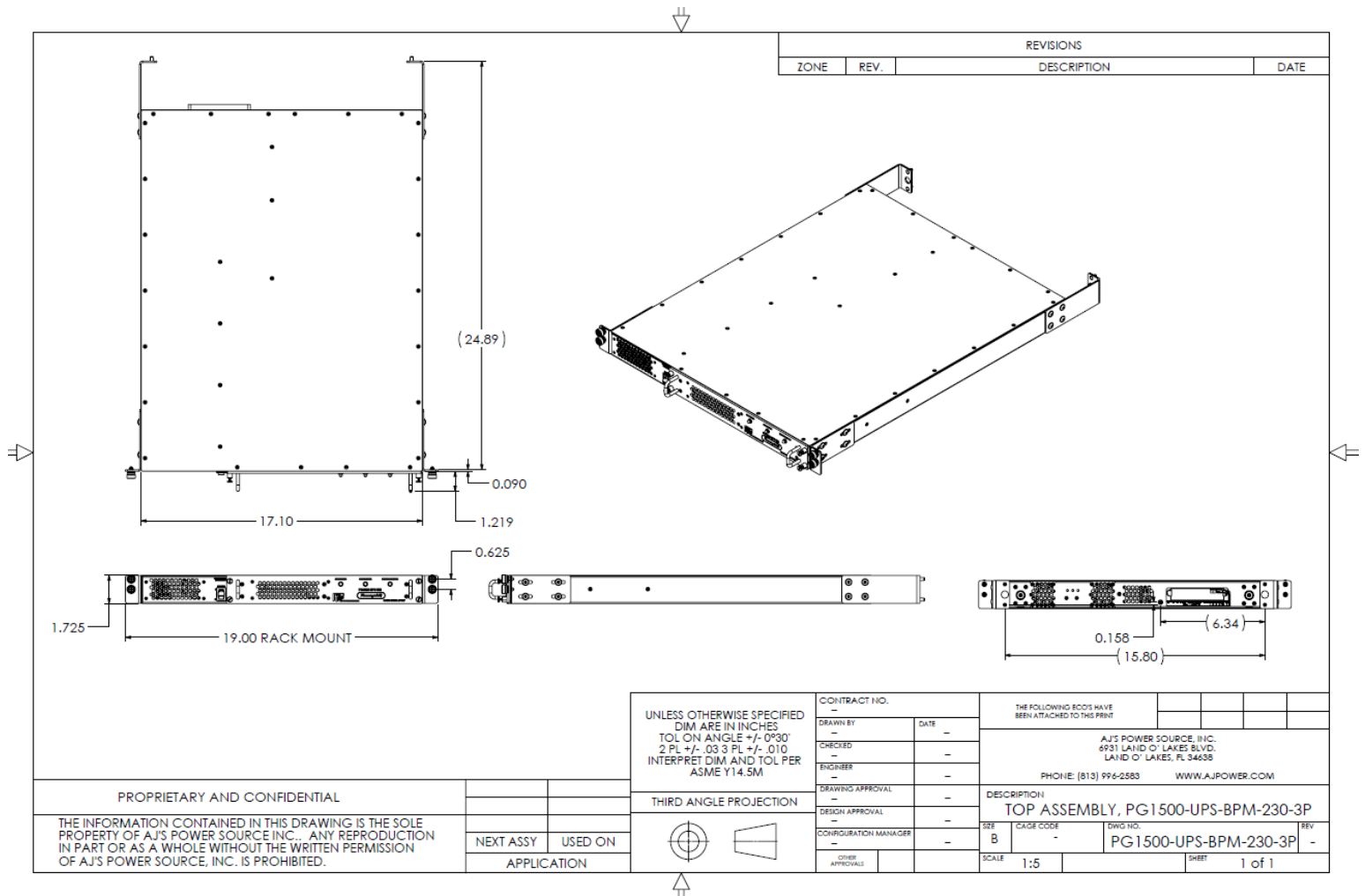
PG1500-UPS-BPM-120 (PG1500-UPS-BPM-230-3P shown) Mechanical View
