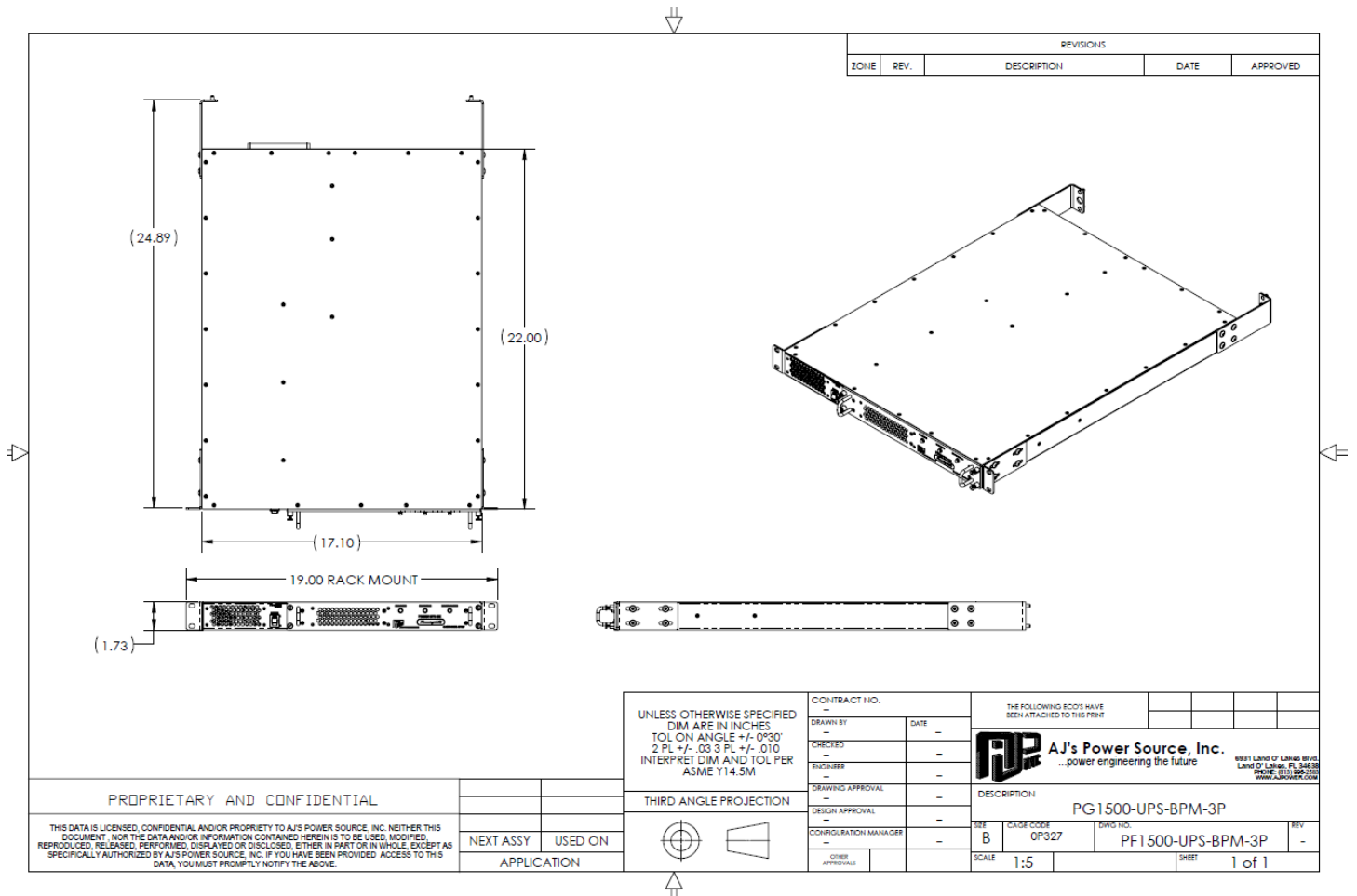
PG1500-UPS-BPM-3P Mechanical View
