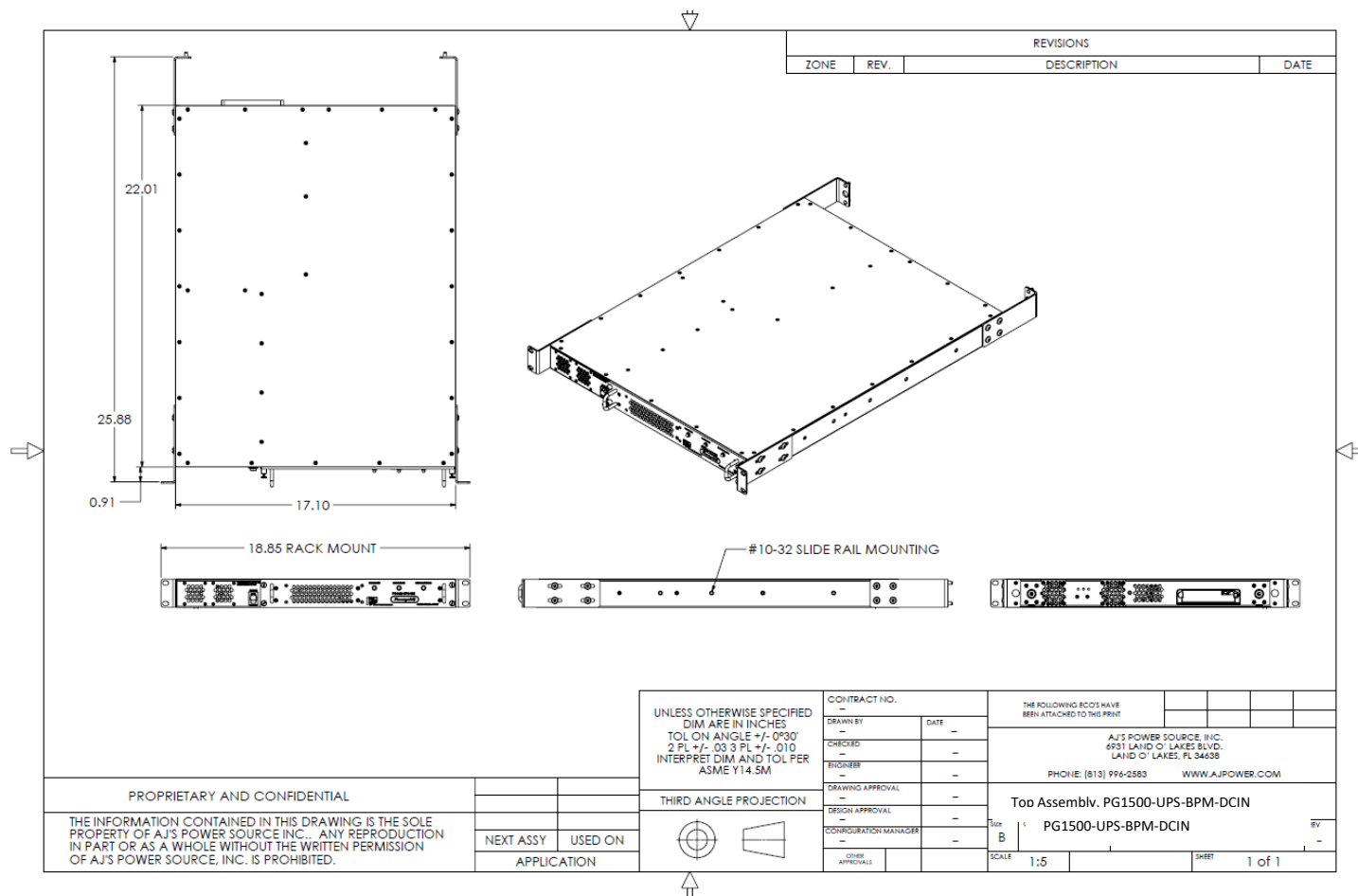
PG1500-UPS-BPM-DCIN Mechanical View
