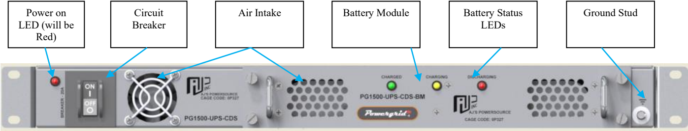
PG1500-UPS-CDS Front View
