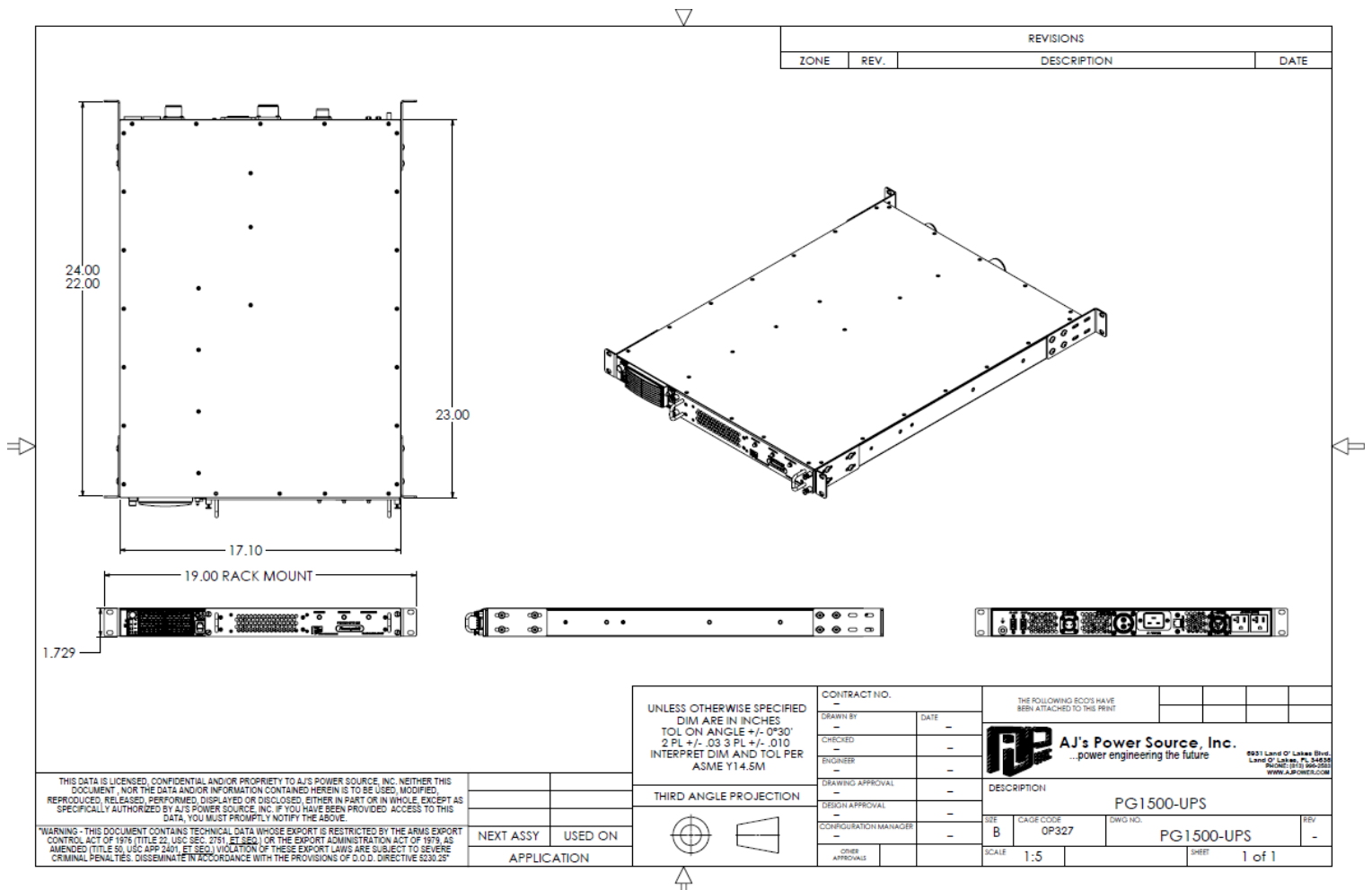
Mechanical Drawing (PG1500-UPS shown, -TMP version mechanically identical)
