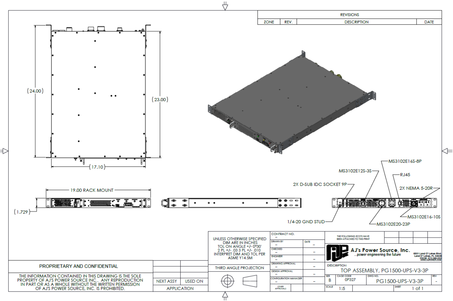
Mechanical Drawing PG1500-UPS-V3-3P shown, PG1500-UPS-V3-3PY same
