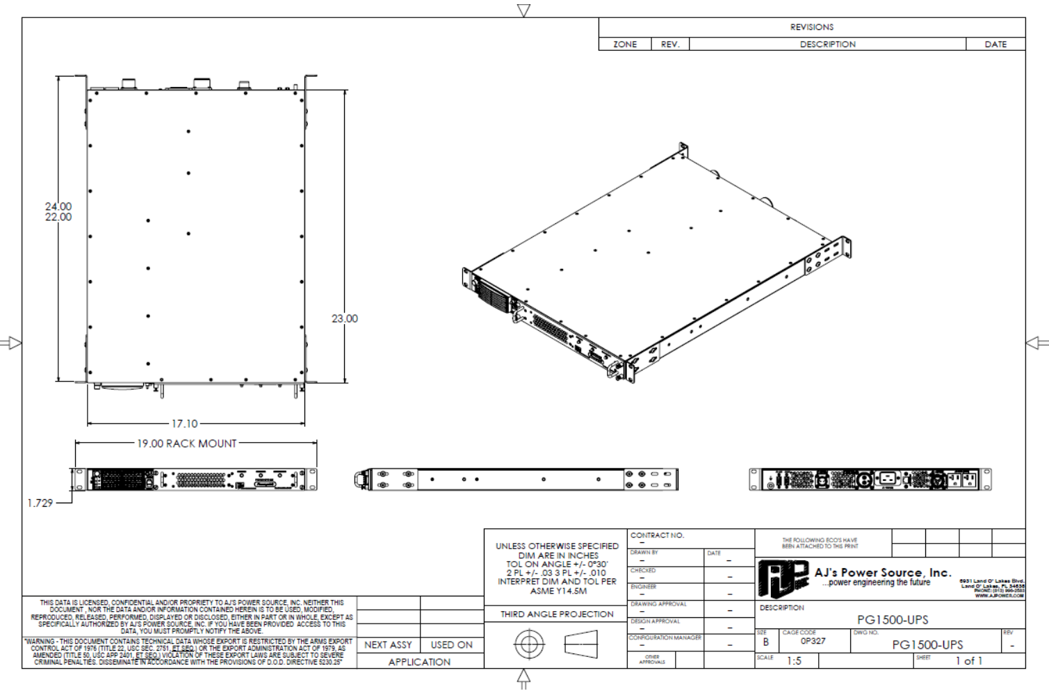
Mechanical Drawing
