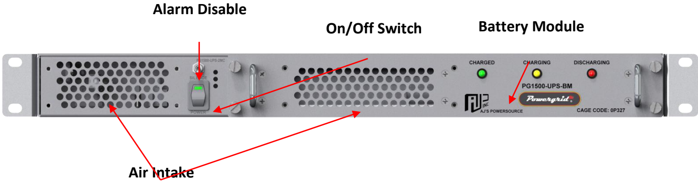
PG1500-UPS-2MC Front View
