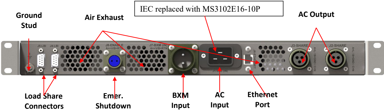
PG1500-UPS-2MC Rear View
